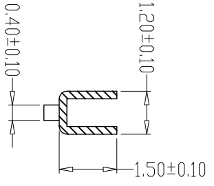
SEC: C-C
